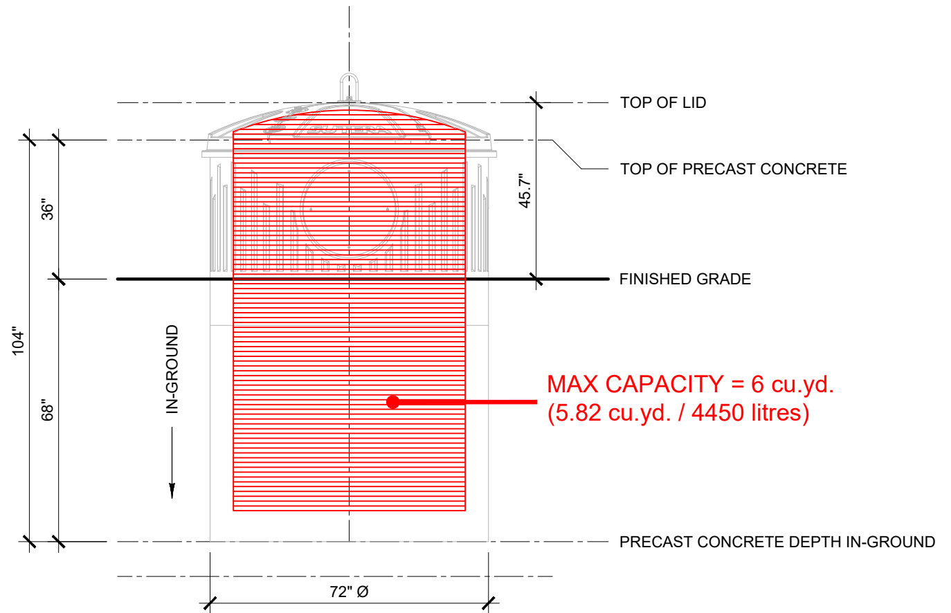
FRONT VIEW
